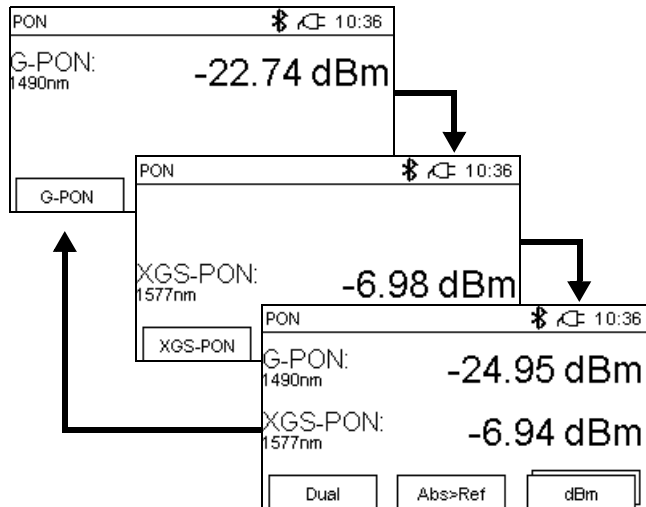
Fig. 4 Operation modes
