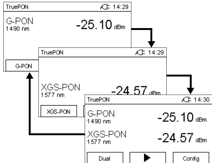
Fig. 5 Operation modes
